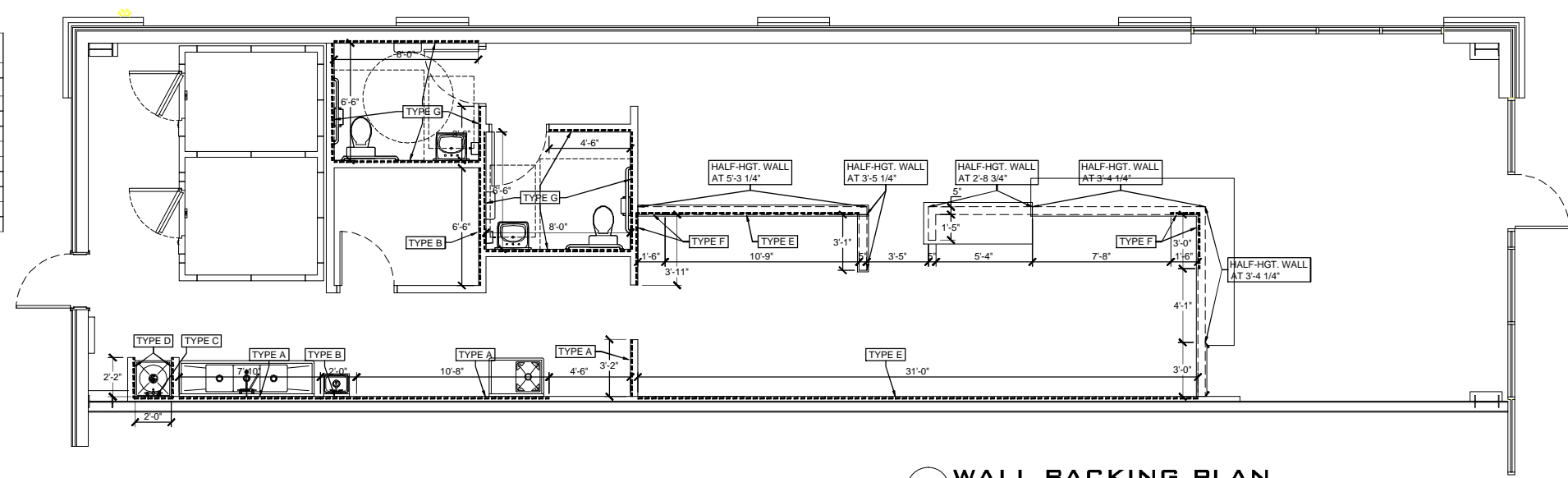
WALL BACKING PLAN SCALE: 1/4" = 1'-0"
