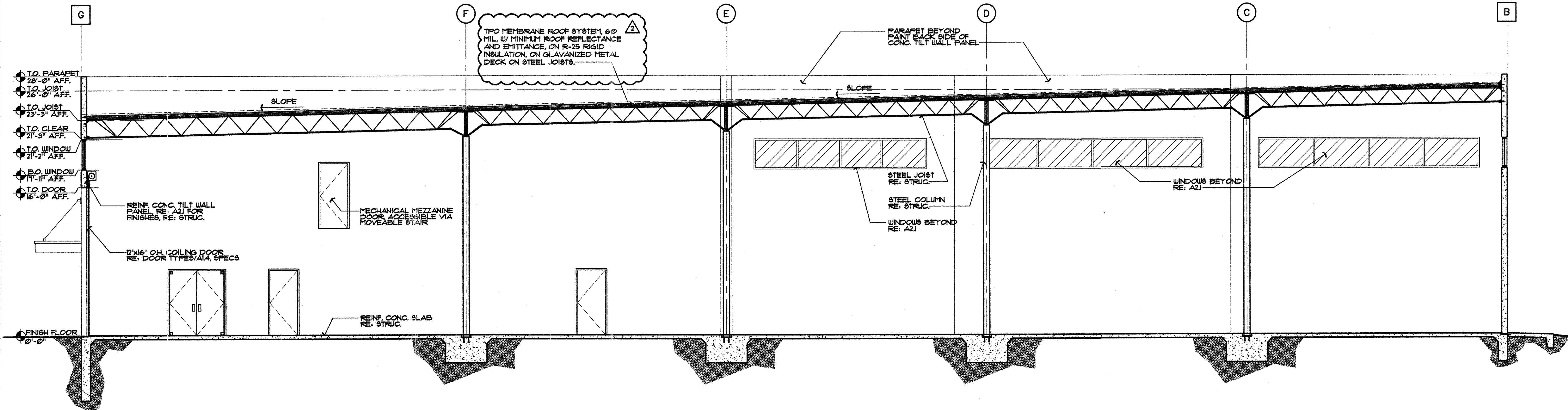
01 BUILDING SECTION - WAREHOUSE SCALE: 3/16" = 1'-0"
