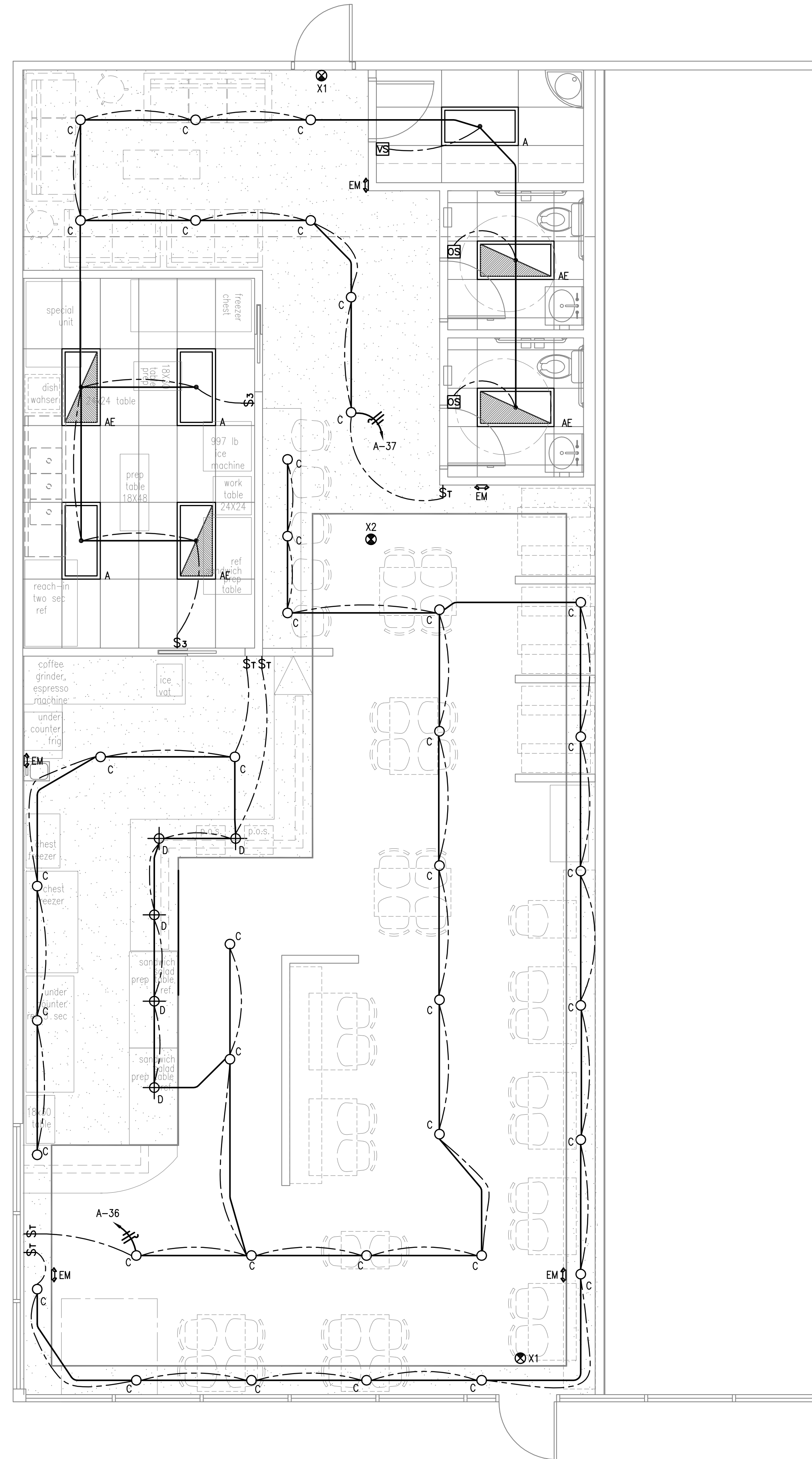
1 ELECTRICAL LIGHTING FLOOR PLAN SCALE: 1/4" = 1'-0"
