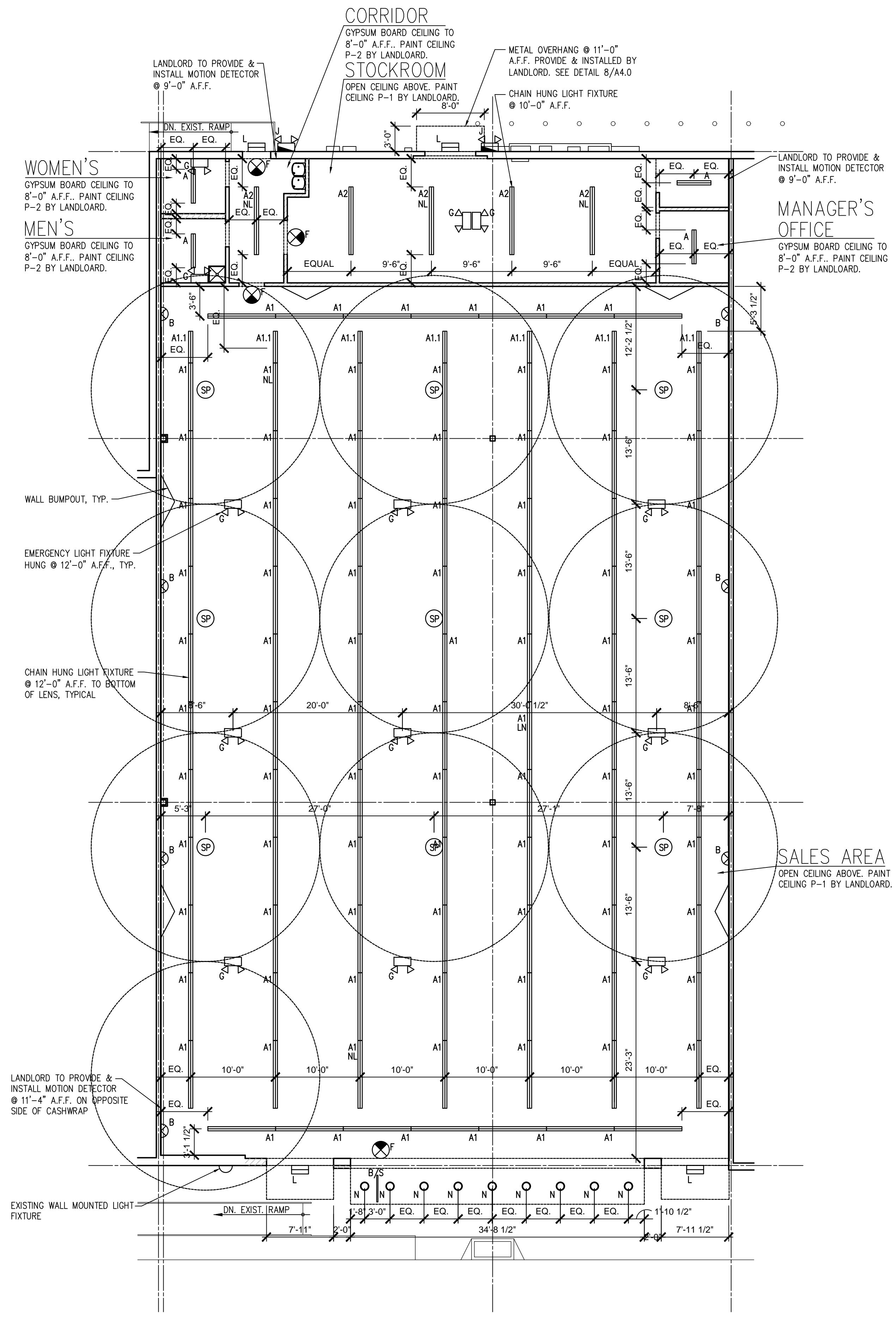
1 REFLECTED CEILING PLAN 1/8" = 1'-0"
