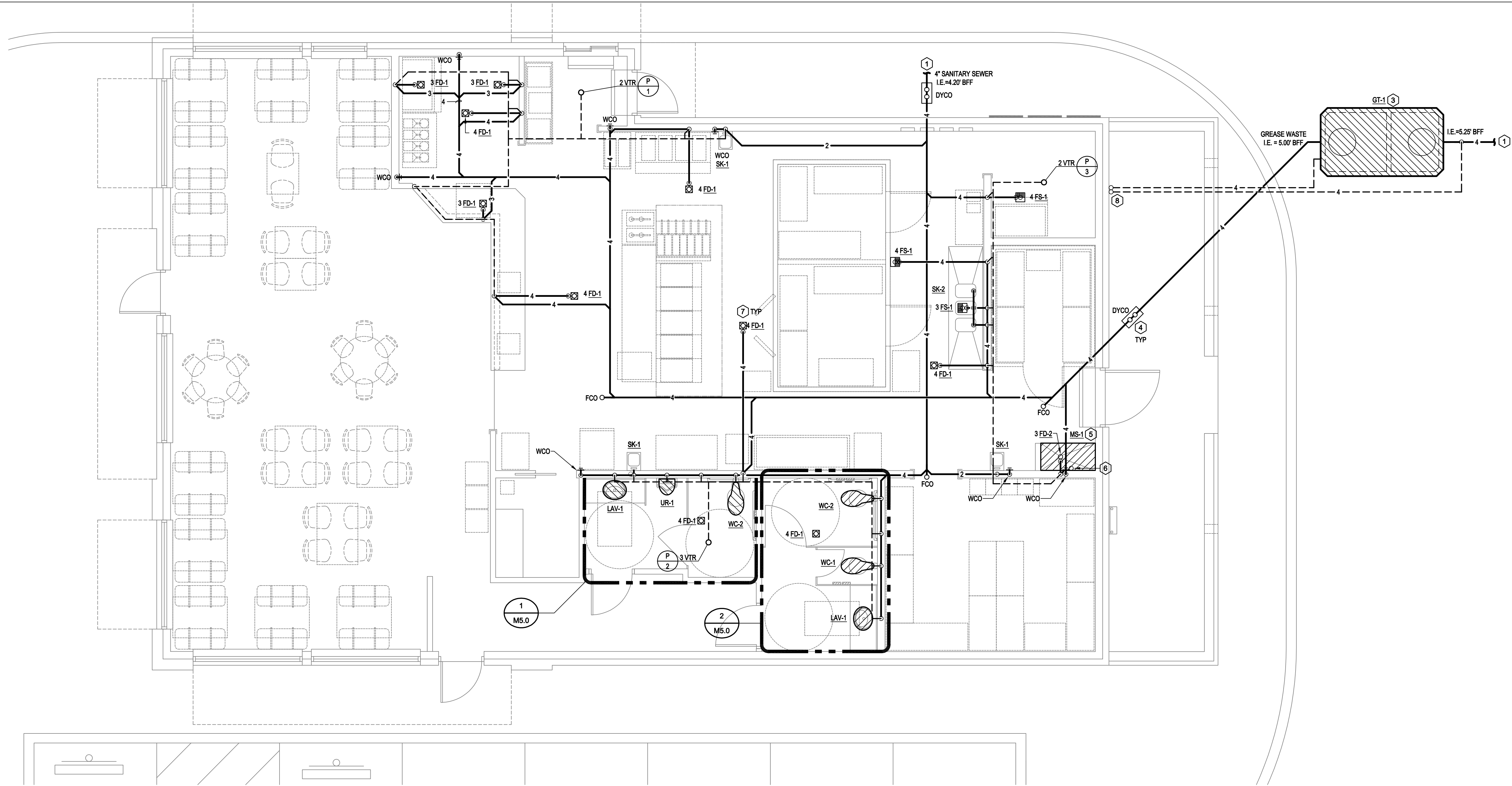
1 PLUMBING FLOOR PLAN - WASTE & VENT SCALE: 1/4" = 1'-0"
