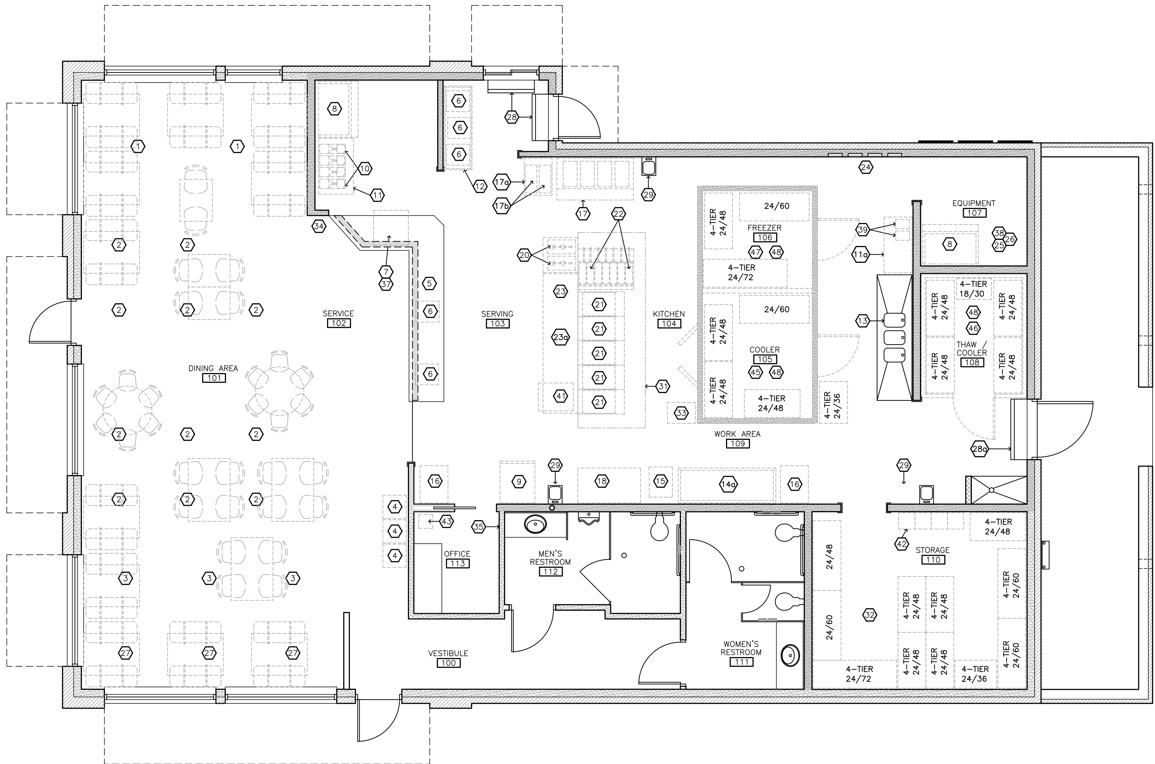
1 EQUIPMENT PLAN SCALE: 1/4" = 1'-0" NORTH
